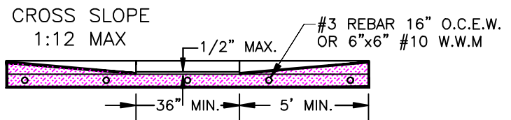
SECTION B-B
